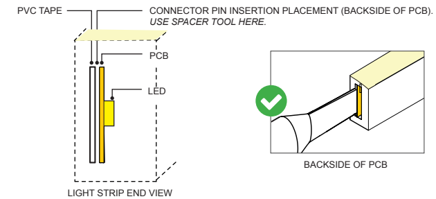
NEVER INSERT SPACER TOOL TO THE FRONT SIDE OF PCB AS THIS CAN DAMAGE THE LEDs.
