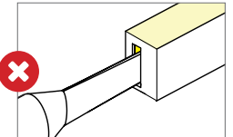
NEVER INSERT SPACER TOOL TO THE FRONT SIDE OF PCB AS THIS CAN DAMAGE THE LEDs.
